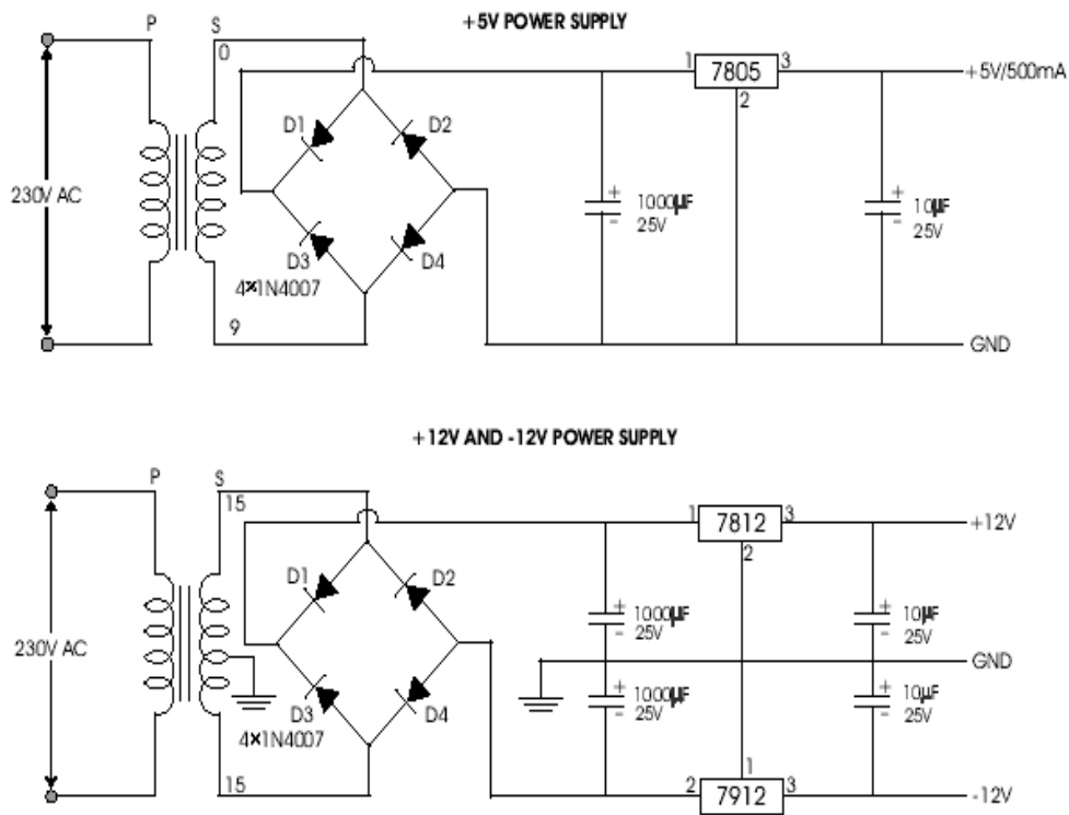
Fig.Circuit Diagram of Power Supply
